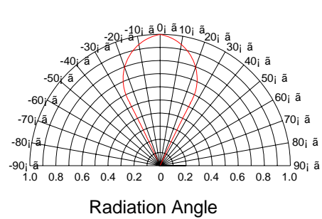
Radiation Characteristics
